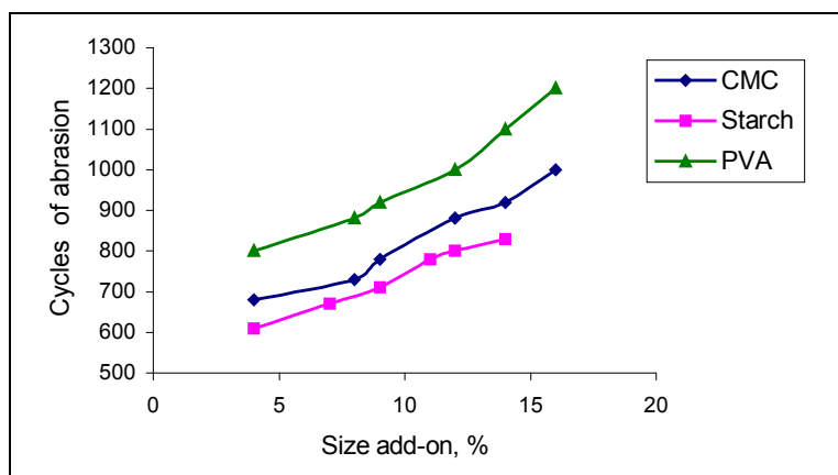
Figure 3. abrasion resistance of yarns sized with different agents.
