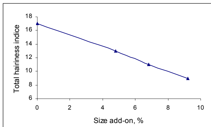
Figure 1. total hairiness indices at different size add-on.
