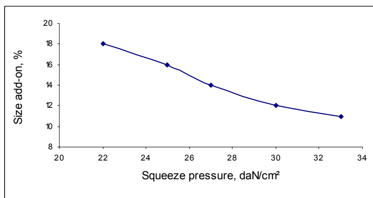
Figure 2. influence of squeeze pressure on size add-on.
